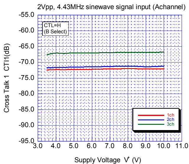
Input Cross Talk 1 vs. Supply Voltage
