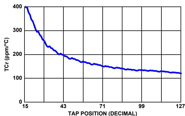
FIGURE 15. 10kΩ TCcr vs TAP POSITION
