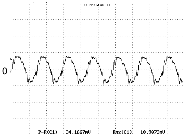
Figure 14: Output voltage ripple at nominal input voltage and rated load current ( I_o=5\text{A} ) (20 mV/div, 2 \mu\text{s}/\text{div} ) Load capacitance: 1\mu\text{F} ceramic capacitor and 10\mu\text{F} tantalum capacitor. Bandwidth: 20 MHz. Scope measurements should be made using a BNC cable (length shorter than 20 inches). Position the load between 51 mm to 76 mm (2 inches to 3 inches) from the module
