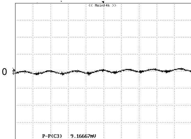
Figure 12: Input reflected ripple current, i_s , through a 12\mu\text{H} source inductor at nominal input voltage and rated load current (20 mV/div, 2 \mu\text{s}/\text{div} )
