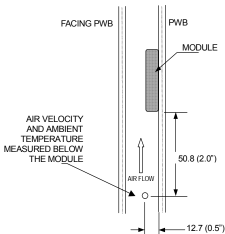
Figure 20: Wind tunnel test setup figure
