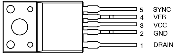
Figure 3. Pin Assignments (Top View)
