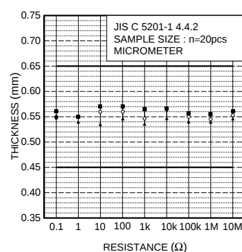
Fig.4 Dimensions (thickness)
