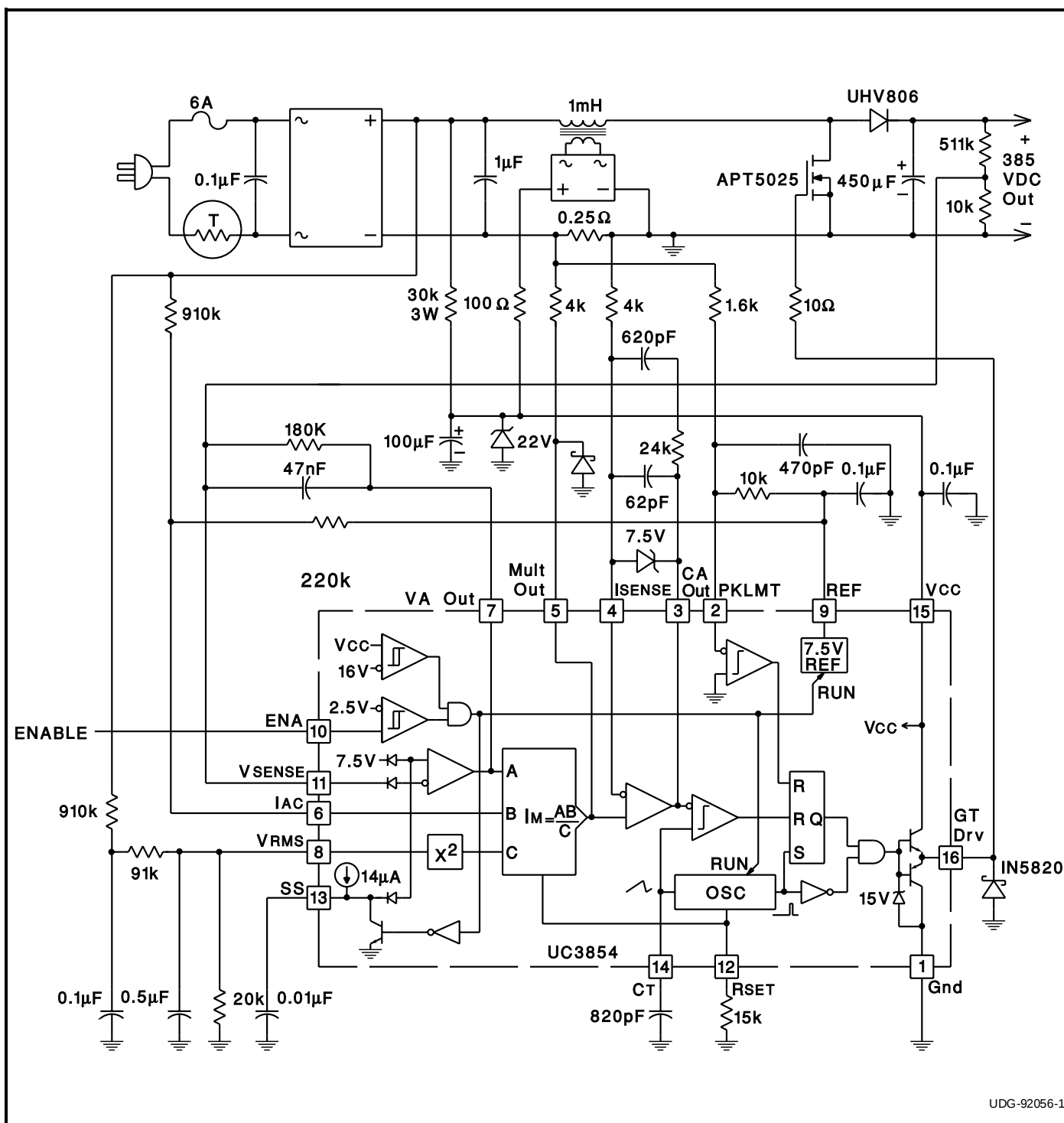
This diagram depicts a complete 250 Watt Preregulator. At full load, this preregulator will exhibit a power factor of 0.99 at any power line voltage between 80 and 260 VRMS. This same circuit can be used at higher power levels with minor modifications to the power stage. See Design Note 39B and Application Note U-134 for further details.
