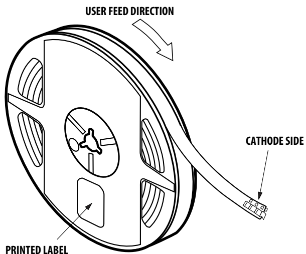
Figure 32. Reeling Orientation
