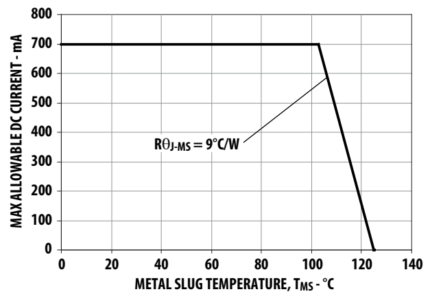
Figure 11. Maximum Forward Current vs. Ambient Temperature. Derated based on T_{JMAX} = 125^\circ\text{C} , R_{\theta MS} = 9^\circ\text{C/W} .
