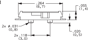
PCM12SMTR SPDT
