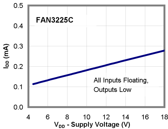
Figure 14. I_{DD} (Static) vs. Supply Voltage (Note 14)
