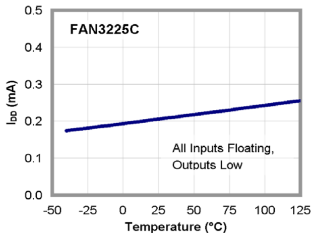
Figure 21. I_{DD} (Static) vs. Temperature (Note 14)
