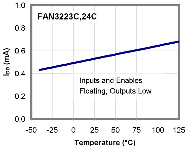
Figure 19. I_{DD} (Static) vs. Temperature (Note 14)
