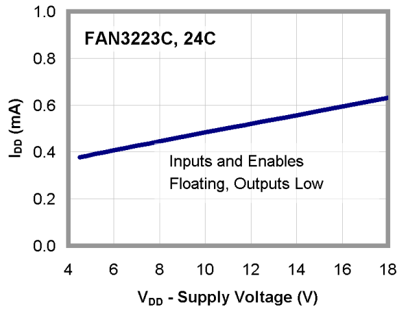
Figure 12. I_{DD} (Static) vs. Supply Voltage (Note 14)
