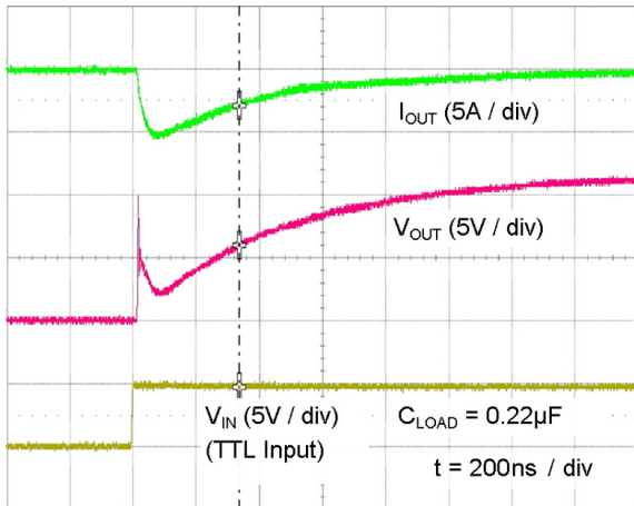
Figure 43. Quasi-Static Source Current with V_{DD} = 12\text{ V} (Note 15)
