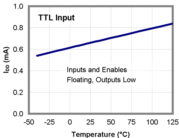
Figure 20. I_{DD} (Static) vs. Temperature (Note 14)
