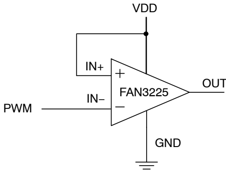
Figure 52. Dual-Input Driver Enabled, Inverting Configuration
