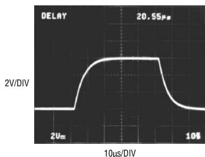
Large-Signal Transient Response G = 100 , V_S = \pm 5V
