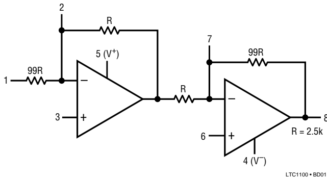
LTC1100 • BD01
