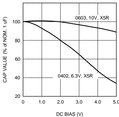
Figure 17. Effect of DC bias on Capacitance Value.
