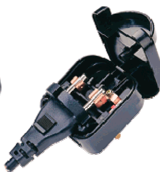
EUROPLUG INSERTED INTO CONVERTER
