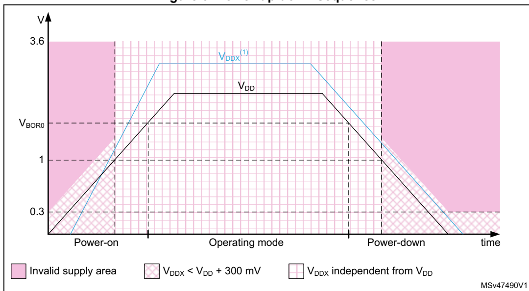
Figure 3. Power-up/down sequence
