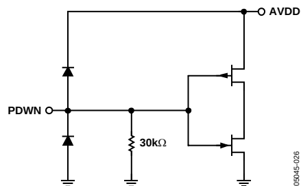
Figure 26. Power-Down Input
