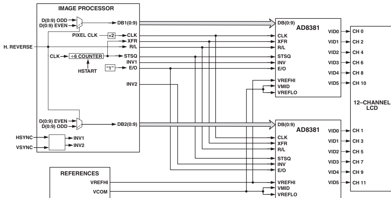
Figure 10. Dual Parallel Data Bus 12-Channel System Block Diagram
