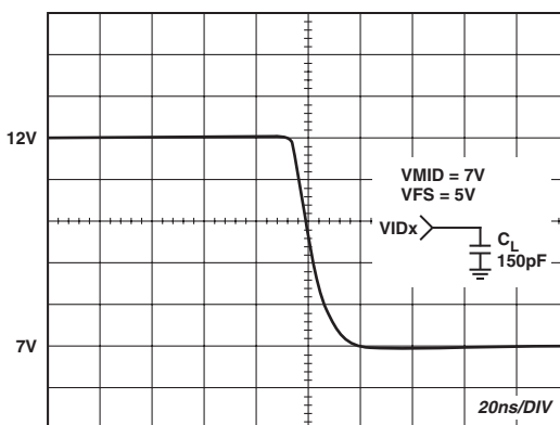
TPC 6. Data Switching 5 V Step Response (Fall) at C_L , INV = H
