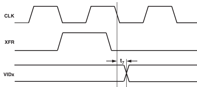
Figure 3. Output Timing
