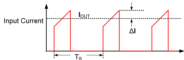
Figure 16. Typical Input Current Waveform.
