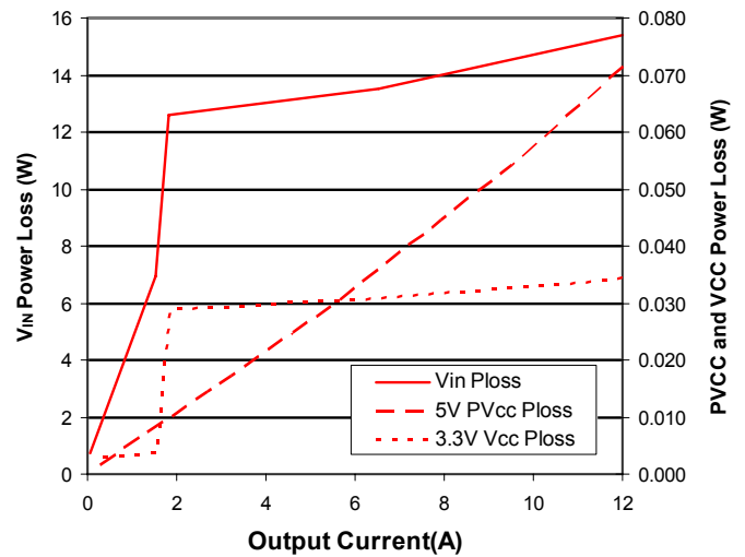
Figure 8. Input Power Vs Output Current
