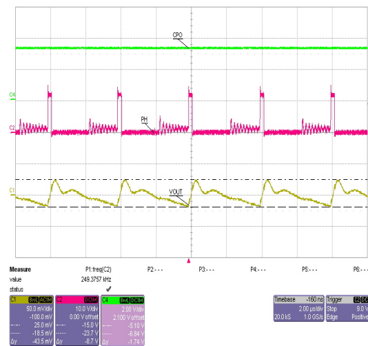
Figure 12: Charge Pump Off at I OUT = 1A
