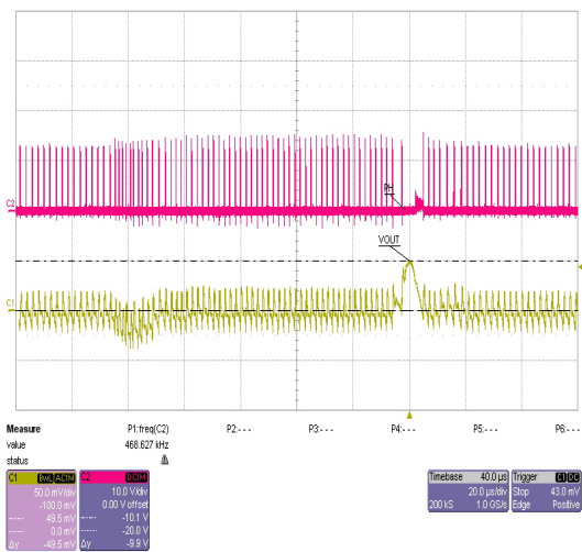
Figure 10: Load Step (2A to 10A) Transient (5A/us) at 12.6V IN : 50mV overshoot, 25mV undershoot
