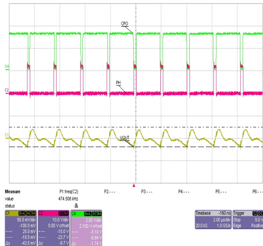
Figure 13: Charge Pump On at I_{OUT} = 3A
