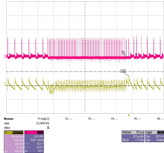
Figure 11: FCCM/CCM transition from 0.5A to 5A at 12.6V IN : 30mV overshoot, 15mV undershoot
