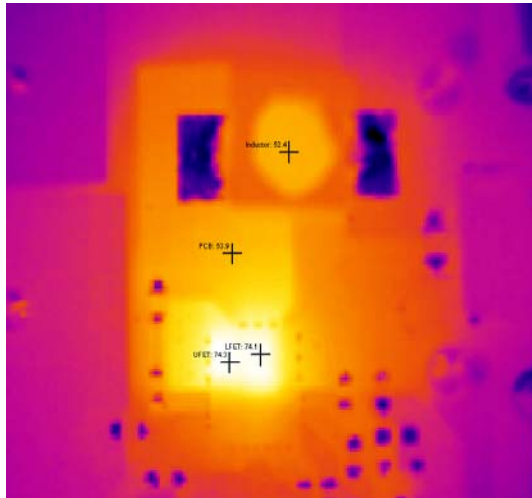
Figure 14: Thermal Image: V_{IN} = 19V , I_{OUT} = 10A , T_a = 25^{\circ}C , no air flow
