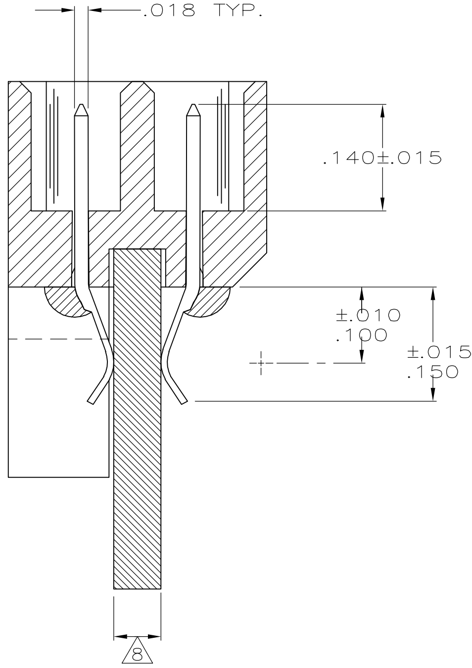
SECTION Y-Y SCALE 8:1 (ROT.90° CW)
