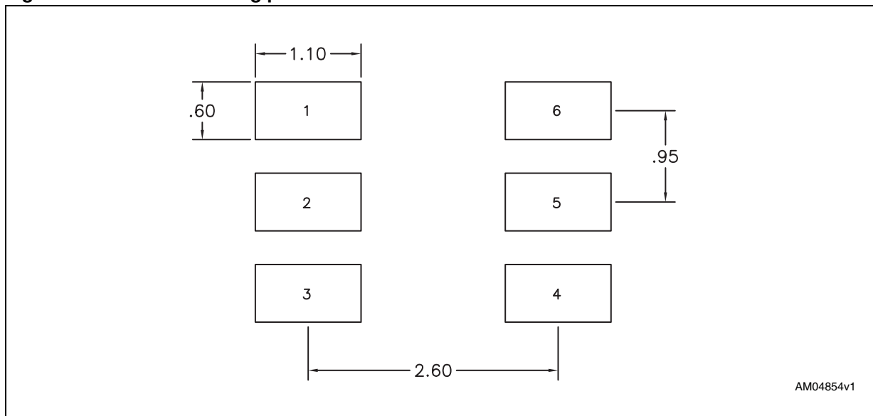
Figure 10. SOT23-6 landing pattern
