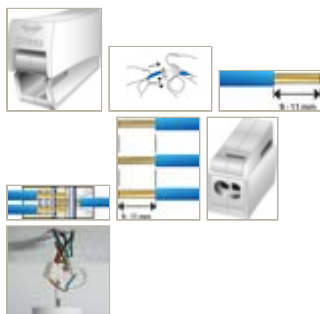
Quick installation and release of lighting devices with HelaCon Lux
