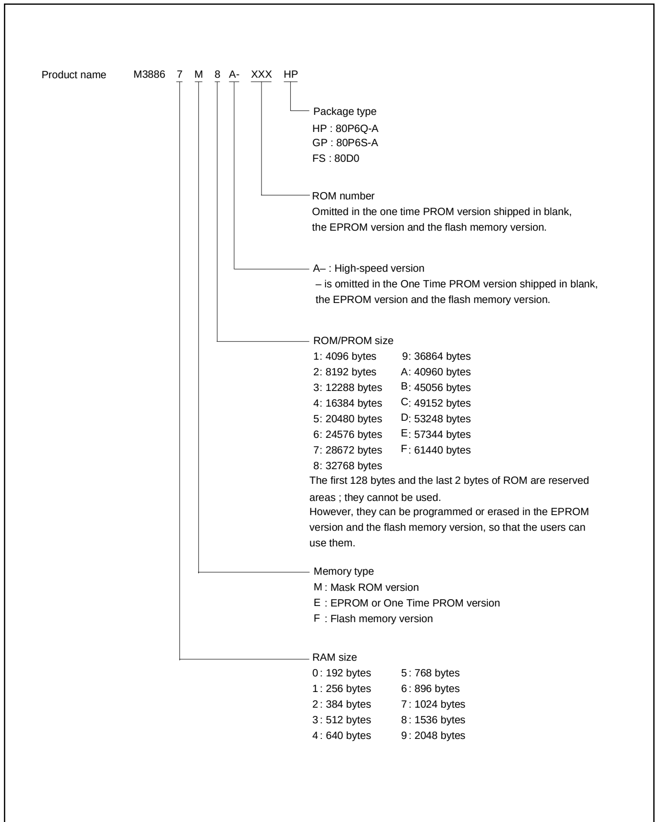
Fig. 5 Part numbering
