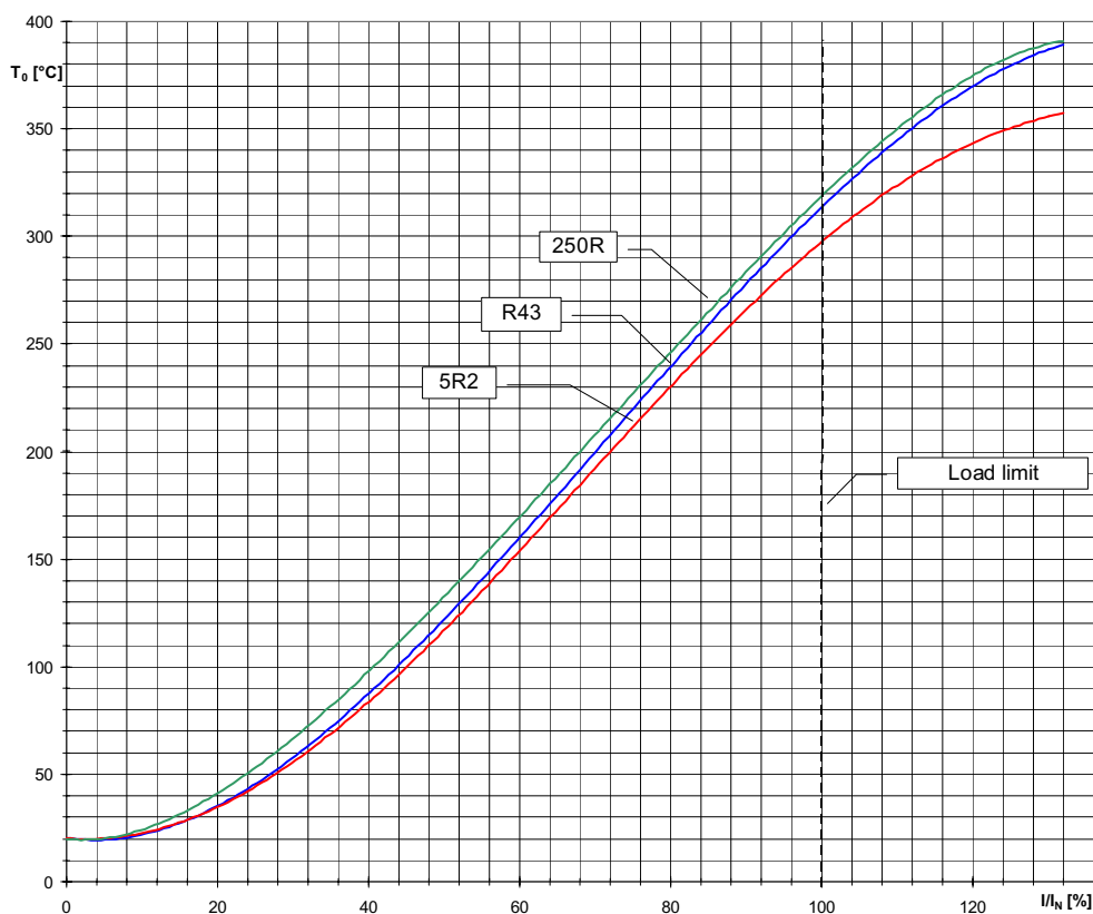
Surface temperature in function of the load
