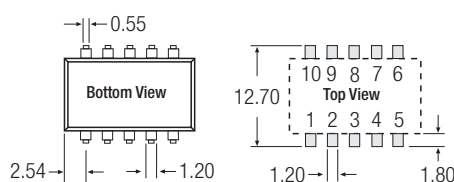
Recommended Footprint Details
