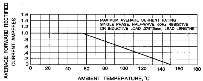
Fig. 3 - FORWARD CURRENT DERATING CURVE
