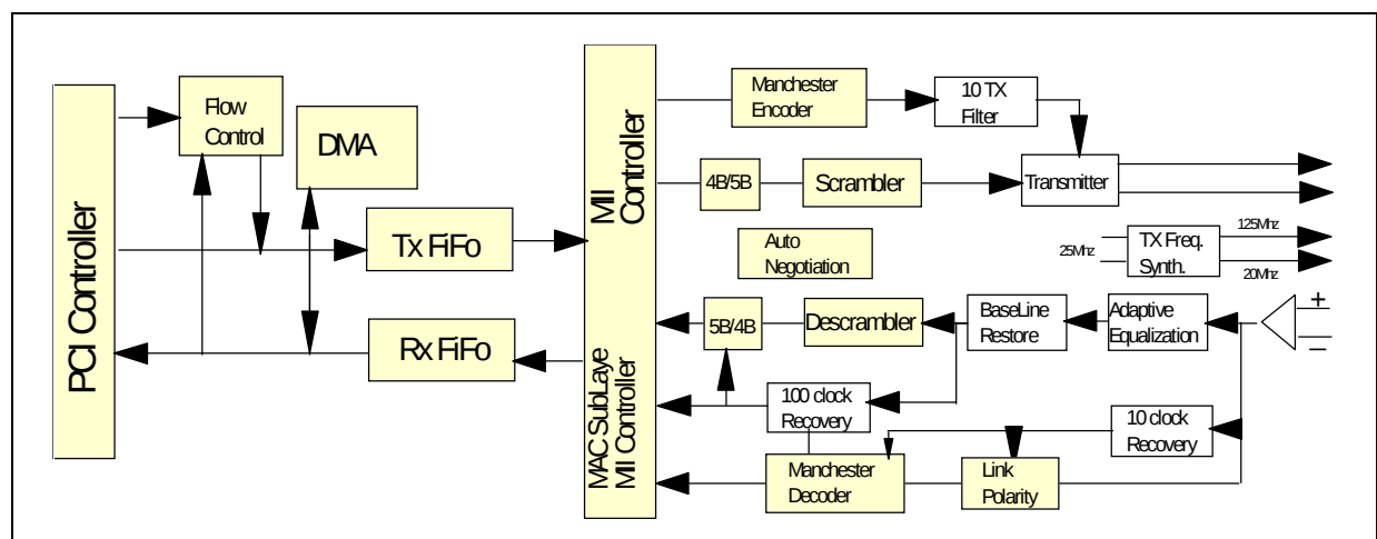
Figure 1. STE10/100Block Diagram
