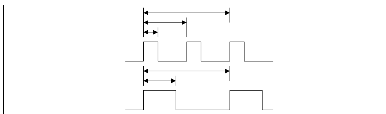
Figure 22. Fast Link Pulse timing
