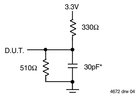
Figure 2. Output Load
