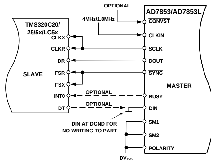
Figure 49. TMS320C20/25/5x Interface
