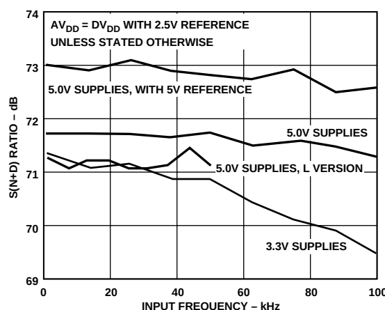
Figure 21. SNR vs. Frequency
