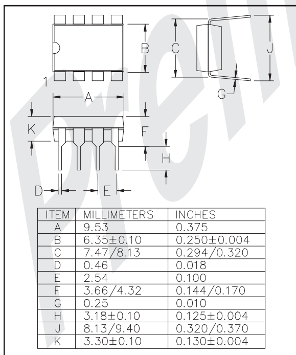
Figure 6. -P (8-pin DIP) version package outline
