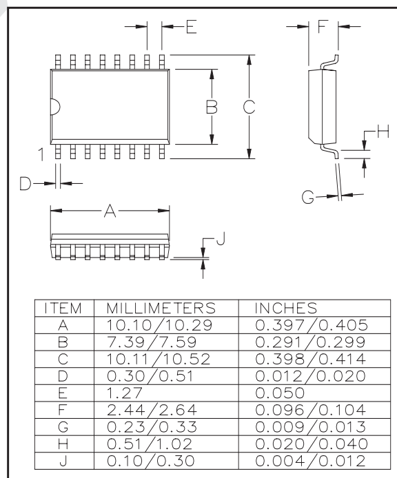
Figure 7. -S16 (16-pin SO) version package outline
