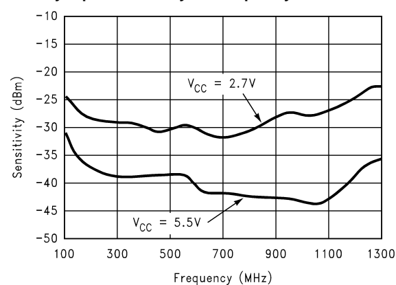
Auxiliary Input Sensitivity vs Frequency
