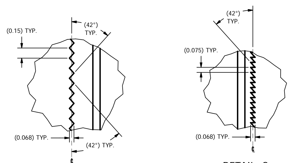
DETAIL F APERTURE LEFT EDGE SCALE 60 : 1
