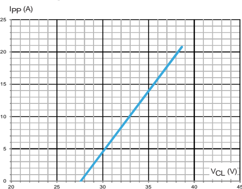
Figure 7: TLP characteristic
