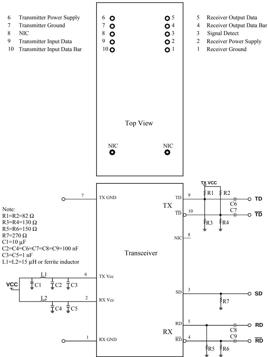
Recommended Circuit Schematic
