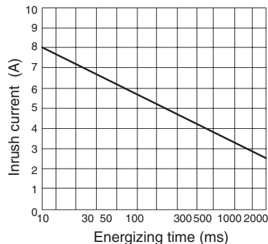
G3R-ODX02SN
