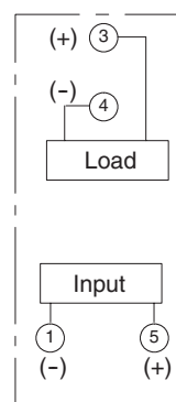
Terminal arrangement/ Internal connections (Bottom view)
