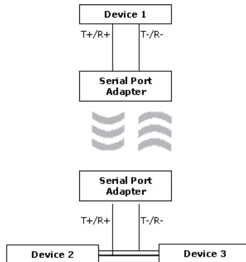
Picture 13. Two-wire RS485 connection setup
