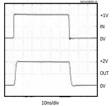
MAX4258/MAX4259 LARGE-SIGNAL PULSE RESPONSE
