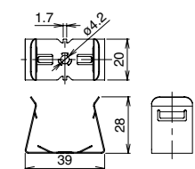
Mounting bracket LF9Z-1SB21
