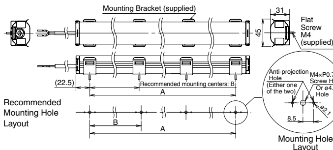
Mounting bracket LF9Z-1SB21
