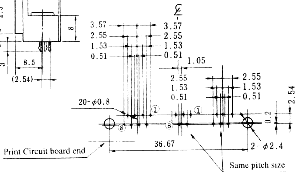
PCB mounting hole layout (Connector mounting side)
