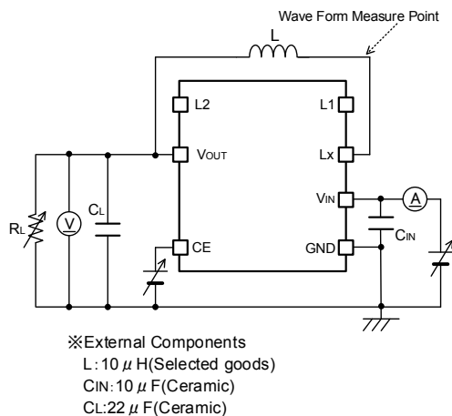
< Circuit No.③ >
