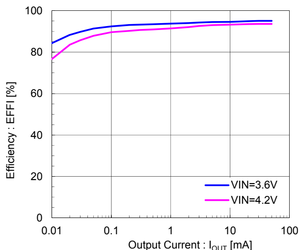
XCL210B301GR-G ( V_{OUT}=3.0\text{V} )
