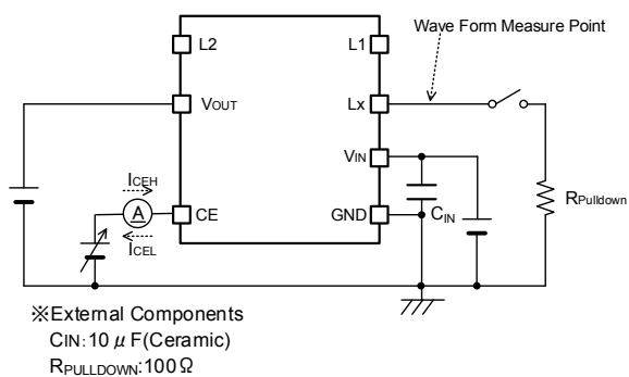
< Circuit No.⑤ >
