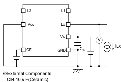
< Circuit No.⑥ >
