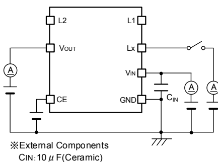
< Circuit No.⑤ >
