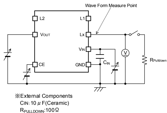
< Circuit No.④ >
