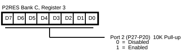
Figure 67. Port 2 Pull-up Register
