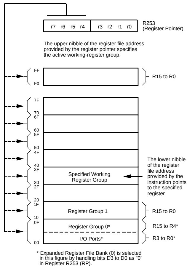
Figure 18. Register Pointer
