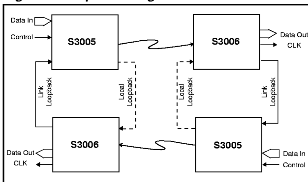
Figure 8. Loopback Diagram
