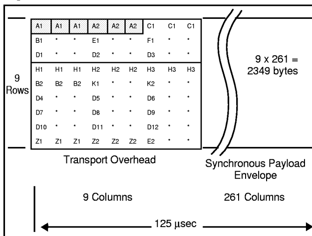
Figure 3. STS-3/OC-3 Frame Format
