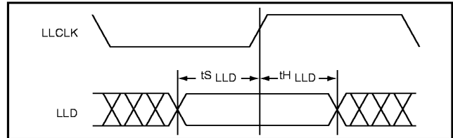
Figure 11. LLD AC Input Timing
