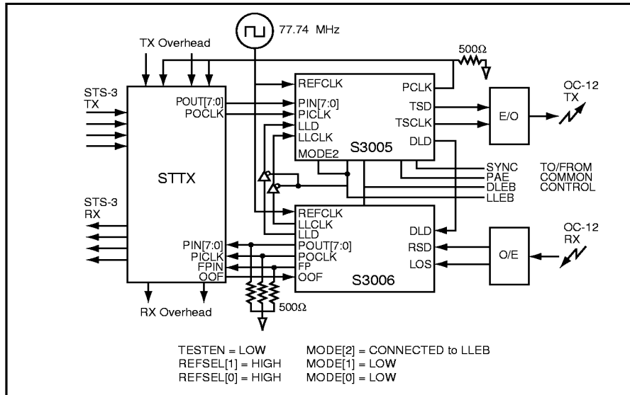
Figure 20. OC-12 Application
