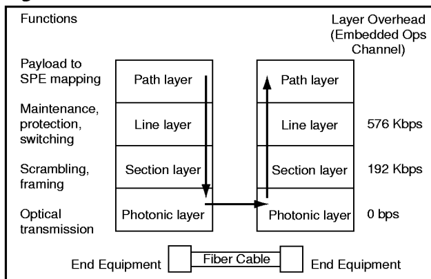
Figure 2. SONET Structure
