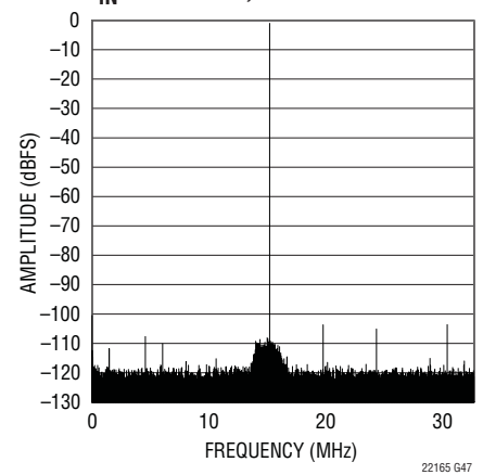
LTC2215 64k Point FFT, f_{IN} = 15.1\text{MHz} , -1dBFS
