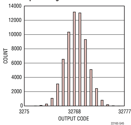
LTC2215 AC Grounded Input Histogram
