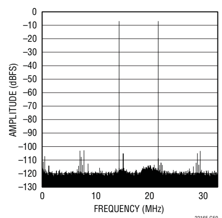
LTC2215 64k Point 2-Tone FFT, f_{IN} = 14.25\text{MHz} and 21.5\text{MHz} , -7dBFS
