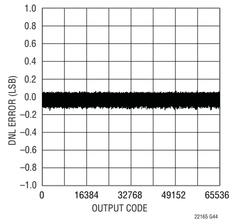
LTC2215 Differential Nonlinearity (DNL) vs Output Code
