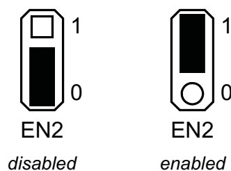
Figure 9. EN2 Jumper Setting
