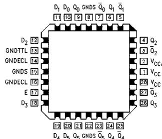
28-Pin PLCC
