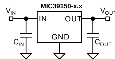
Figure 1. Capacitor Requirements
