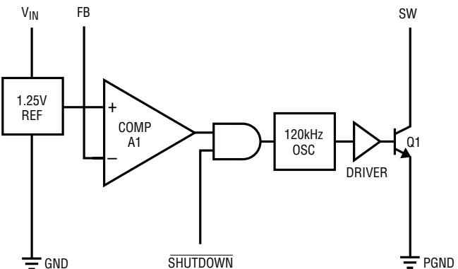
LT1109A (Adjustable)
