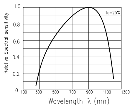
Fig.2 Spectral Sensitivity
