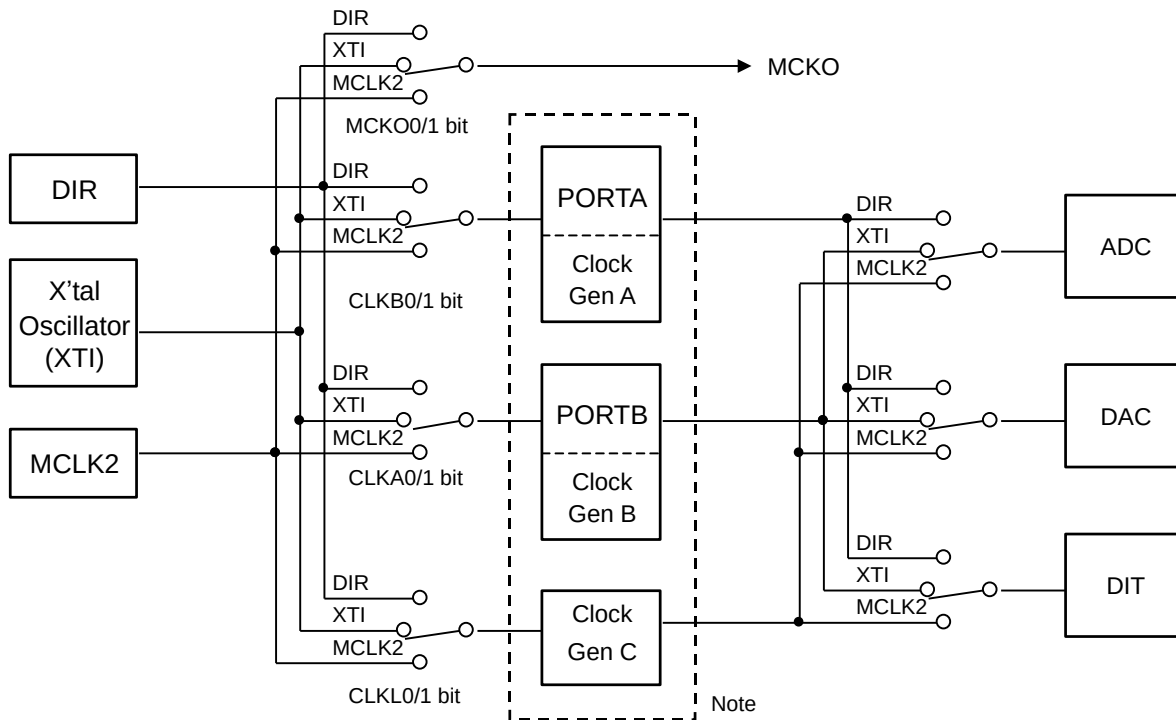
Figure 2. System Clock
