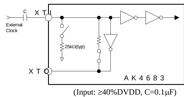
Figure 5. AC-coupled Input
