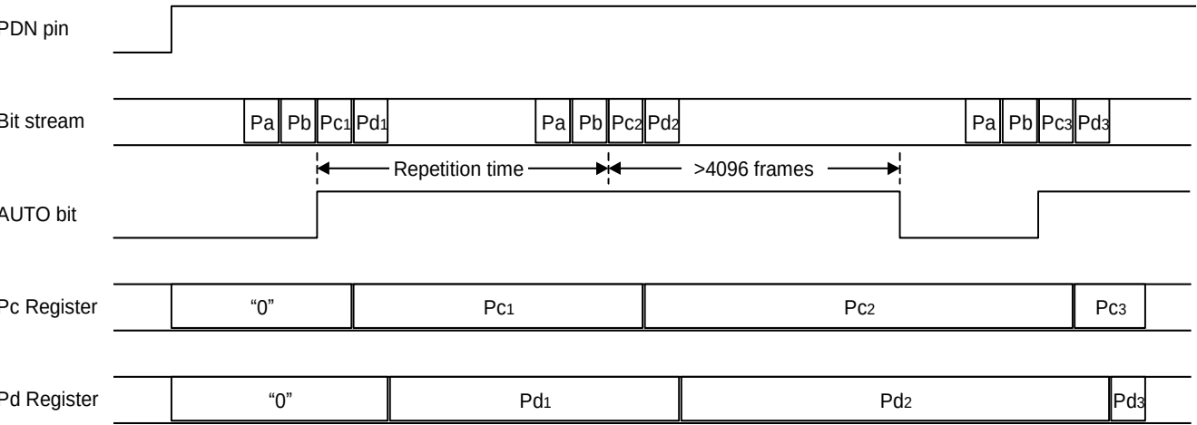
Figure 38. Timing example 1
