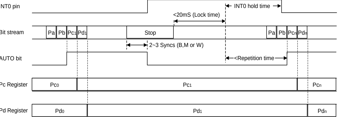
Figure 39. Timing example 2
