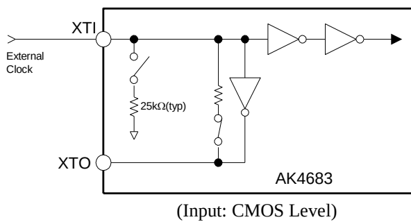
Figure 4. DC-coupled Input
