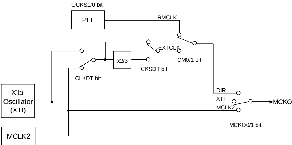
Figure 7. MCKO Clock
