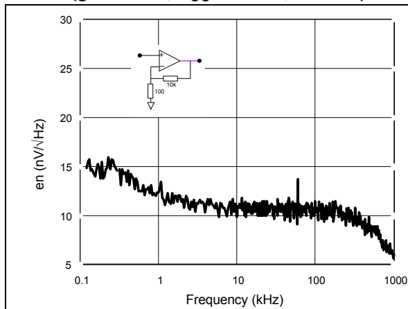
Figure 27. Equivalent noise voltage (gain = 100, V_{CC} = \pm 2.5 V, no load)
