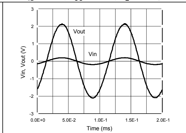
Figure 28. Maximum output swing (gain = 11, V_{CC} = \pm 2.5 V, R_L = 150 \Omega )
