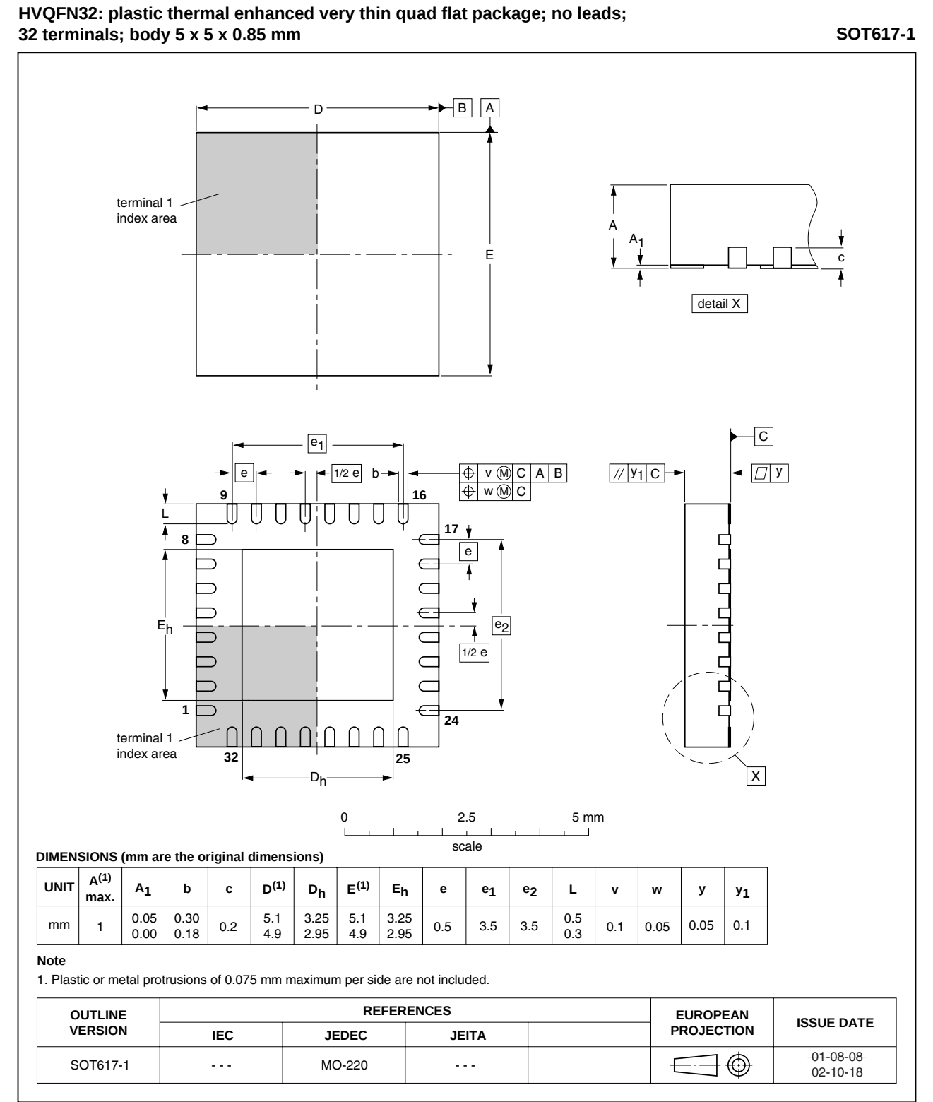
Fig 15. Package outline SOT617-1 (HVQFN32)
