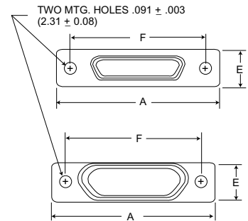
Solder Pot
