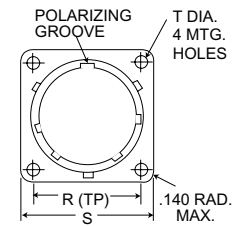
RECEPTACLE ASSEMBLY
