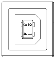
SERIES "B" USB JACK J1
